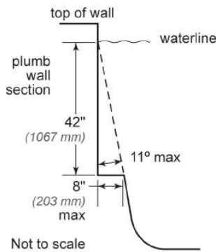
Figure 4 Offset ledges
